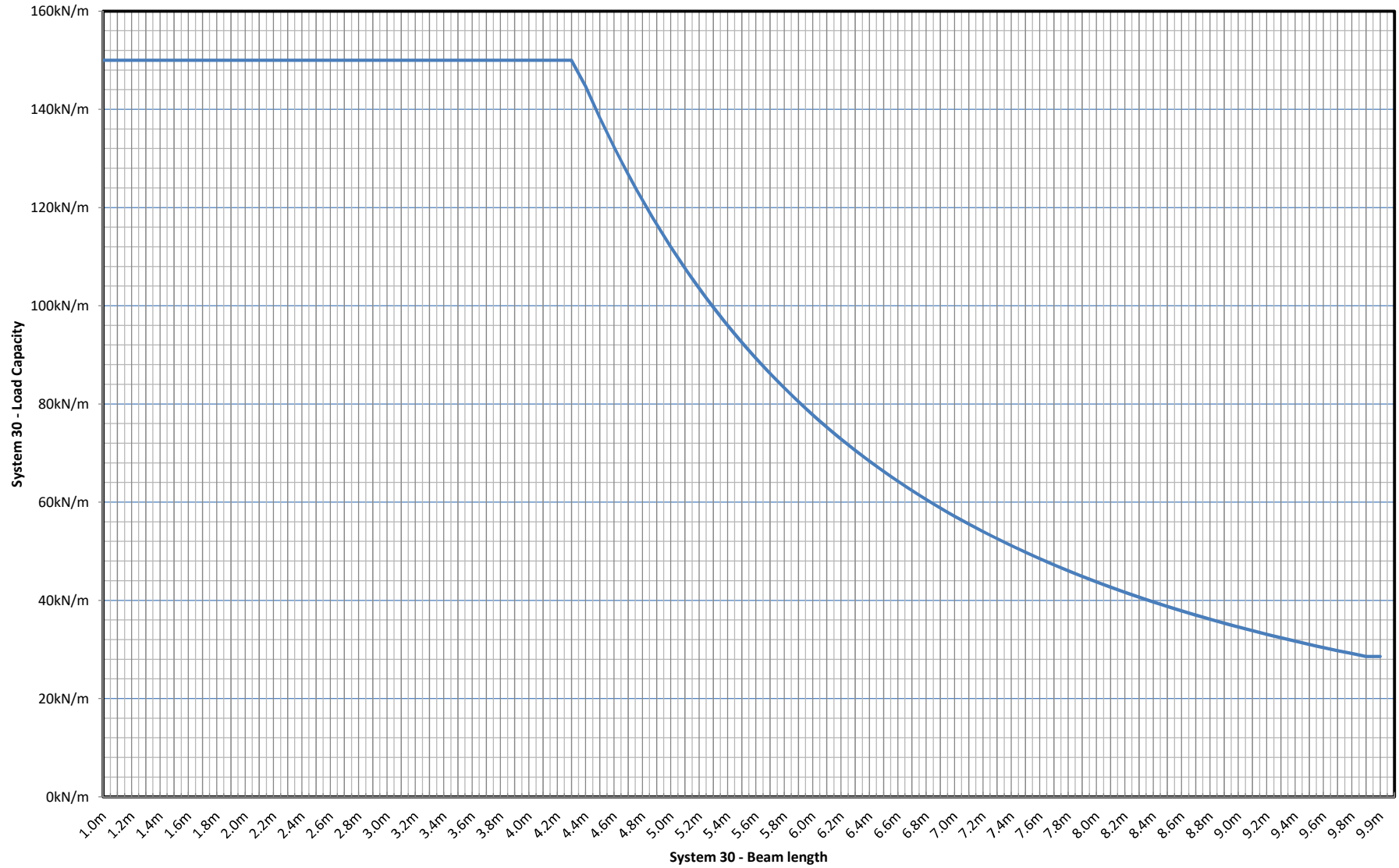
System 30 - Allowable Loading (kN/m)
